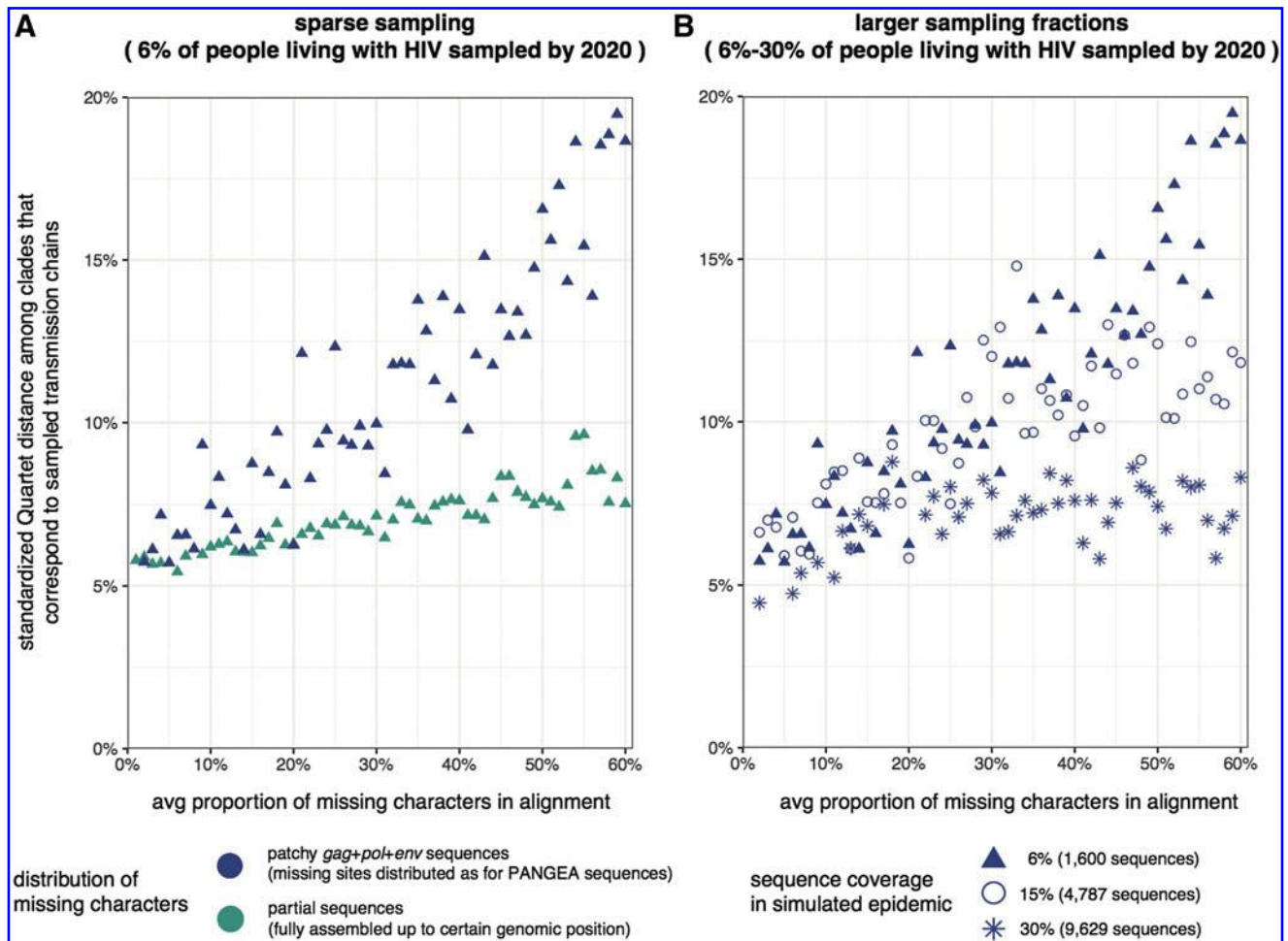
FIG. 4. Excess negative impact of irregularly distributed missing characters on HIV-1 phylogeny reconstruction. Four times 60 sequence alignments of varying size (1,600 to 9,629 sequences, shape of points) and varying missing site patterns (either patchy or allocated in a single block after a certain genome position, color of points) were simulated (data sets D1-Mxx, D4-Mxx, D5-Mxx, D6-Mxx, D1-Pyy, see Supplementary Table S1). For each alignment, the average proportion of missing characters per sequence in alignments relative to the length of the gag+pol+env genome (6,807 nt) was calculated. One phylogeny per alignment was reconstructed with RAxML. (A) We first compared Quartet distances of trees reconstructed from patchy sequence alignments of 1,600 taxa to those of trees reconstructed from partial sequence alignments of 1,600 taxa. For the same average number/average proportion of missing characters, viral trees were less accurately reconstructed when missing characters were irregularly distributed. (B) We then compared Quartet distances of trees reconstructed from patchy sequence alignments of that increased in the number of viral sequences sampled. The excess error in Quartet distances associated with irregularly distributed missing characters vanished as sampling coverage approached 30% of individuals living with HIV-1 by 2020 in the simulations (~10,000 taxa).
