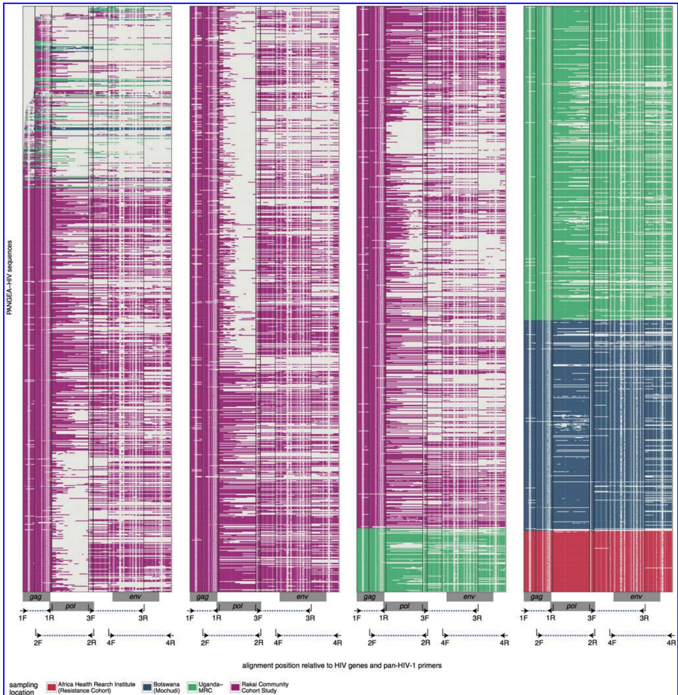
FIG. 1. Alignment of the first PANGEA-HIV consensus sequences. Three thousand nine hundred eighty-five HIV-1 consensus sequences were generated from samples collected as part of the Mochudi Prevention Project ( dark blue ), the Rakai Community Cohort Study ( purple ), the Africa Health Research Institute Resistance Cohort ( red ), and the general population, fisherfolk, and female sex worker cohorts from MRC/UVRI Uganda ( green ). Locations of the HIV-1 gag , pol , and env genes are indicated on the x -axis, along with the primer sets of the Gall protocol that were used to amplify four overlapping genomic regions ( arrows and blue dots ). Vertical lines indicate the position of primers in the alignment. Missing data and gaps are shown in white . The total length of the alignment is 9,742 nt and covers the viral genome between HIV-1 gag and nef (length 8,628 nt in reference strain HXB2).
